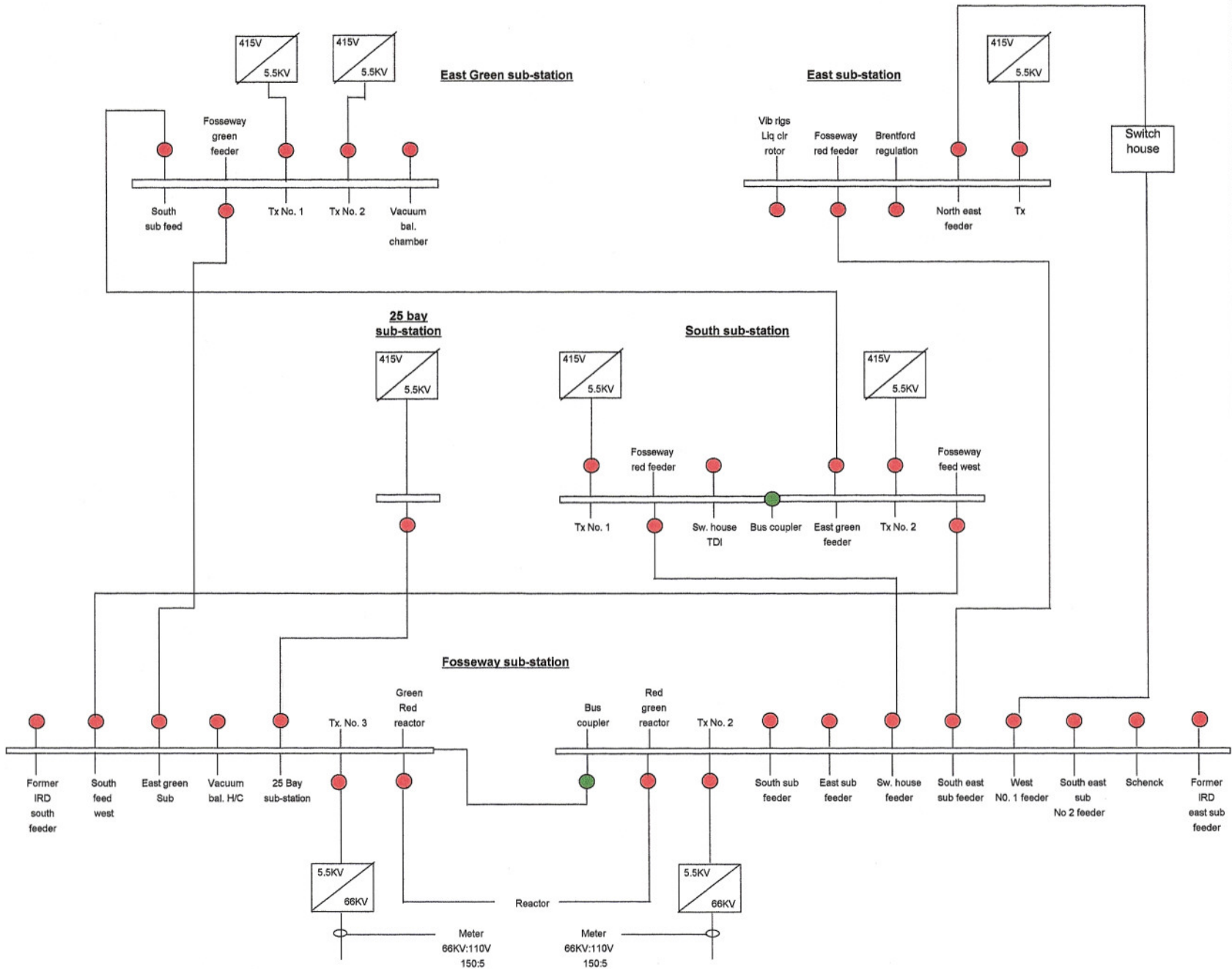
WORKS 5.5KV SCHEMATIC (Fig. 2)
